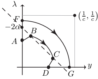
Fig. 4. Construction of the x -increment map X_1 when (1 + 2\alpha c) > 0 .
