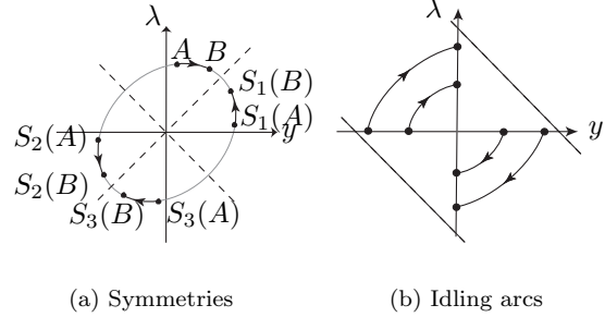
Fig. 3. (a) Discrete symmetries in the linear region. (b) Idling arcs.
