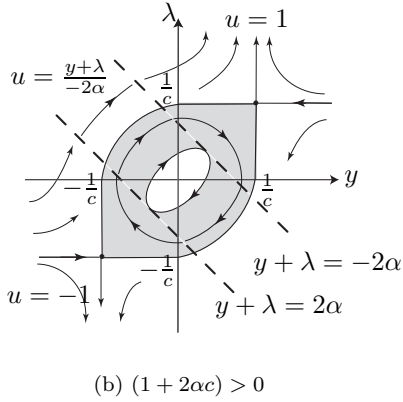
Fig. 2. The phase portrait in the y\lambda -plane when \lambda_x > 0 and (1 + \alpha c) > 0 . Depending on the sign of (1 + 2\alpha c) , point (0, -2\alpha) is above or below point (0, 1/c) on the \lambda axis.
