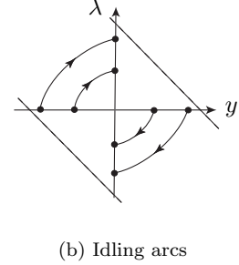
Fig. 3. (a) Discrete symmetries in the linear region. (b) Idling arcs.
