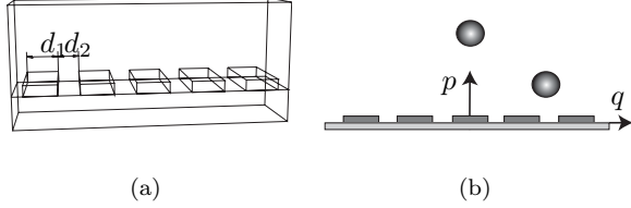
Fig. 1. The dielectrophoretic system is a chamber filled with a fluid medium where there is a parallel array of electrodes at the bottom.
