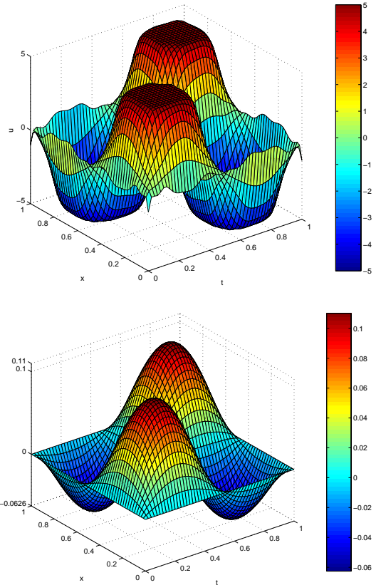
Fig. 2. Example. Optimal control (up) and state (down).
