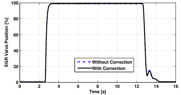
(a) EGR Valve position
