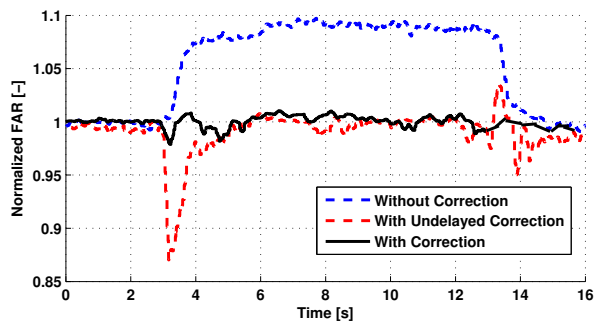
(b) Normalized Fuel-to-Air Ratio
